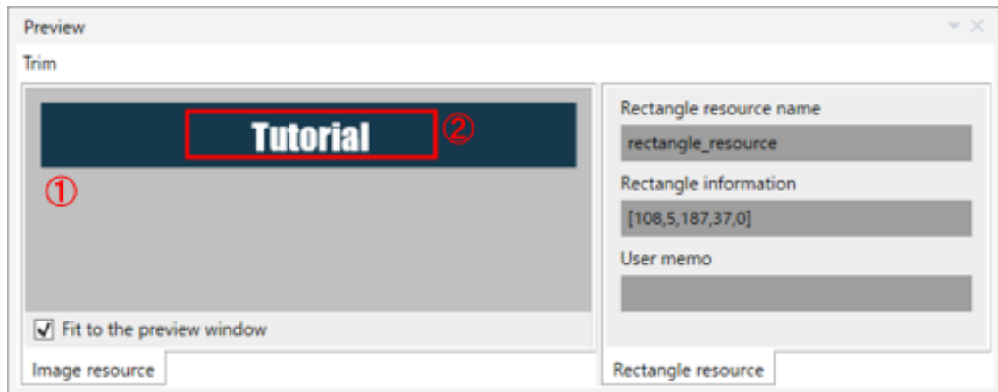
Figure 10-16 Main tab (“Rectangle resource” is specified as the input.)
