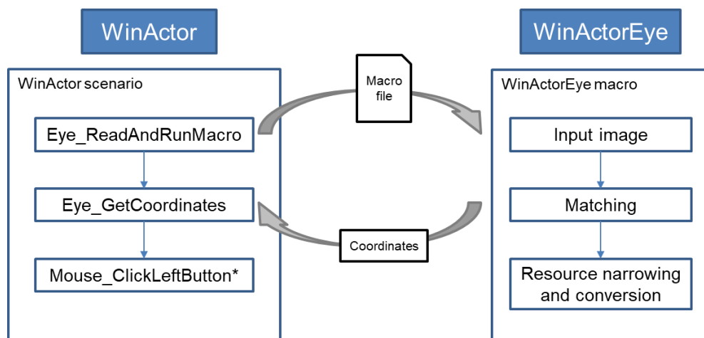
Figure 2-1. Relationship diagram between WinActorEye and WinActor
